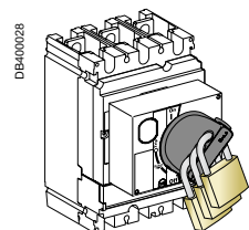
Rotary-handle locking using a padlock or a keylock.
