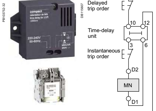
MN release with a time-delay unit.
