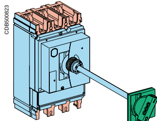
EasyPact CVS400/630 with extended rotary handle
