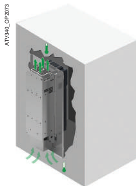
Flange-mounting kit installed inside cabinet
