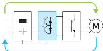
3-level technology
