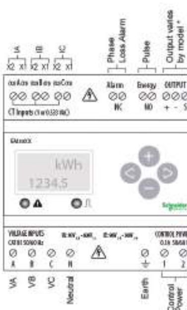
EM3502/EM355x parts and connection terminals
