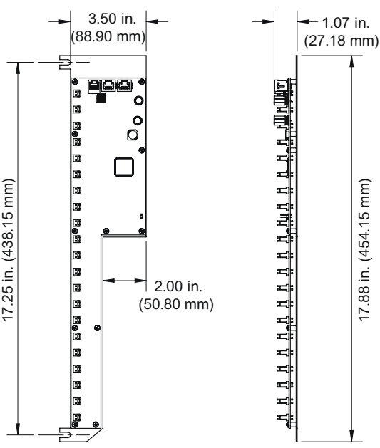
Right strip - top and side views
